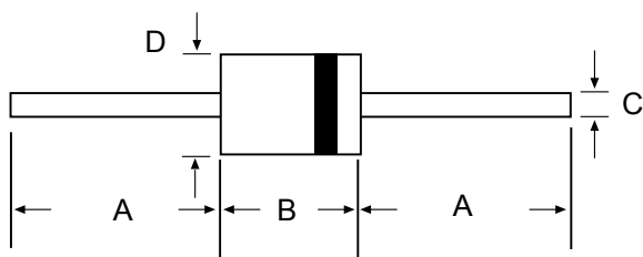
DO-201
