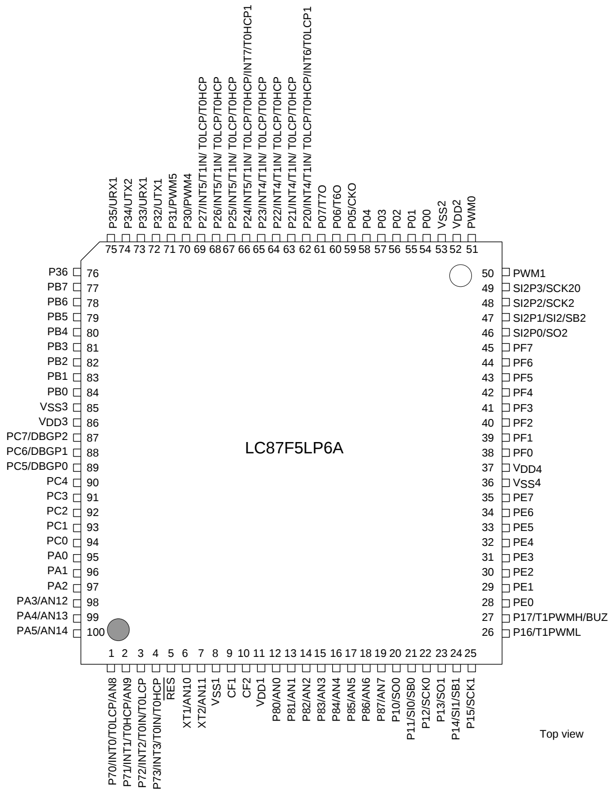
TQFP100(14×14) “Lead-free Type”
