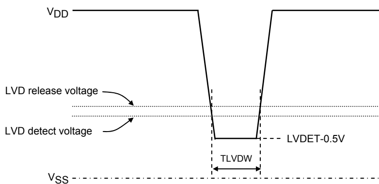
Figure 10 Minimum Low Voltage Detection Width (Example of Voltage Sag/Fluctuation Waveform)
