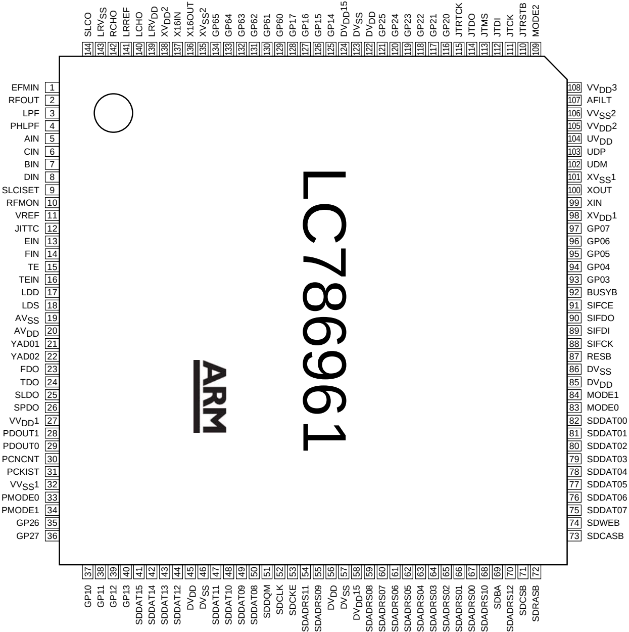
Top view
