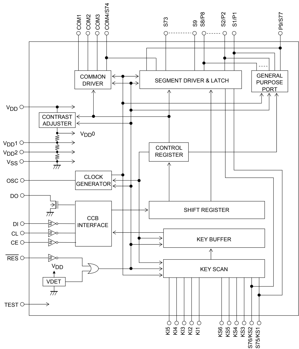
Block Diagram
