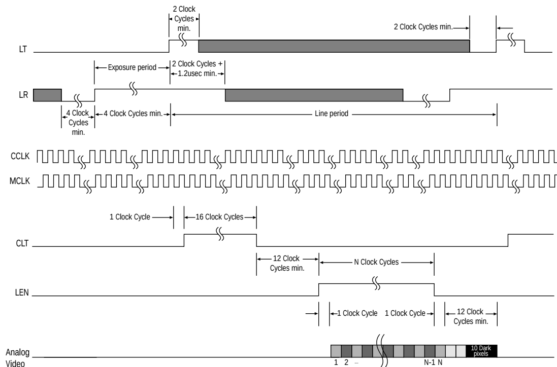
Figure 4: Slave Mode Timing Diagram
