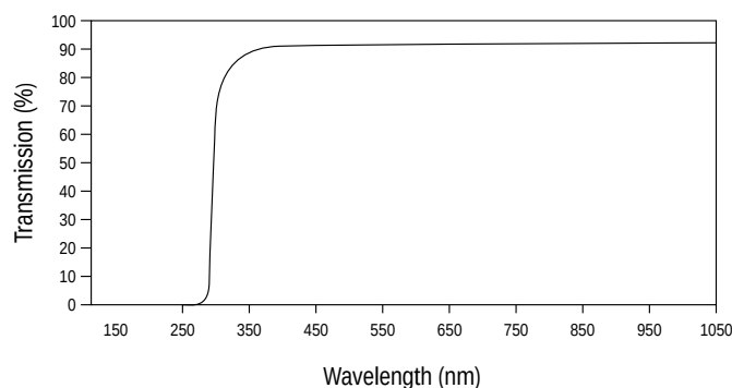
Figure 1b: Sensor Window Transmission Curve
