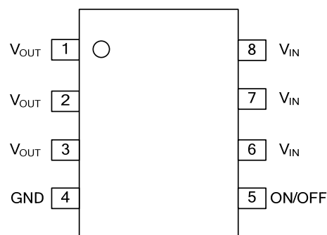
SOP-8
