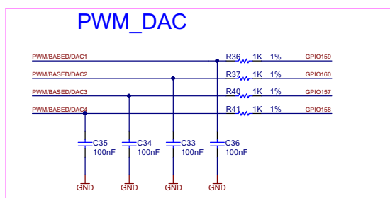
Figure 6. P05_PWM-DAC
