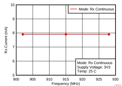
Figure 31. Rx Current vs Frequency - 915 MHz
