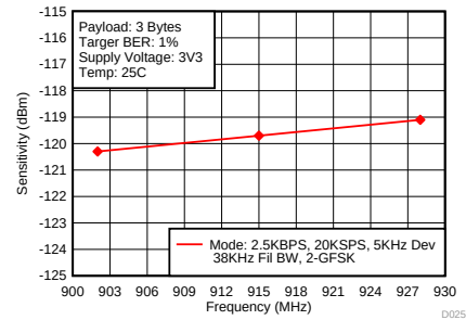
Figure 28. Rx Sensitivity vs Frequency in LRM – 915 MHz Band
