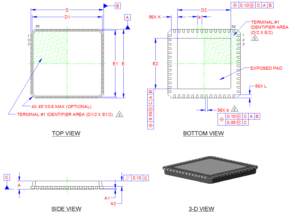
Figure 2 56-Pin QFN Package Definition
