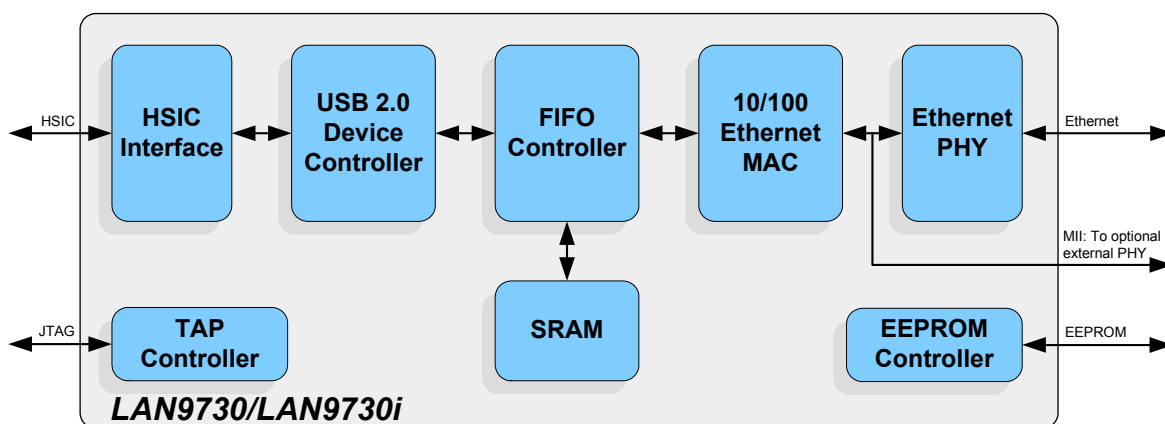
Figure 1 LAN9730/LAN9730i Block Diagram
