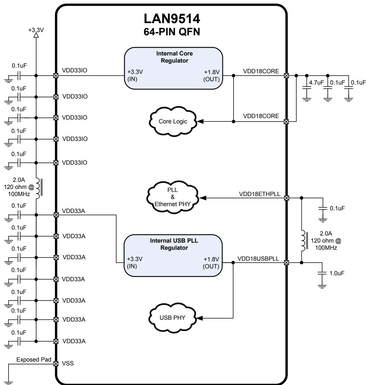
FIGURE 2-2: POWER CONNECTIONS
