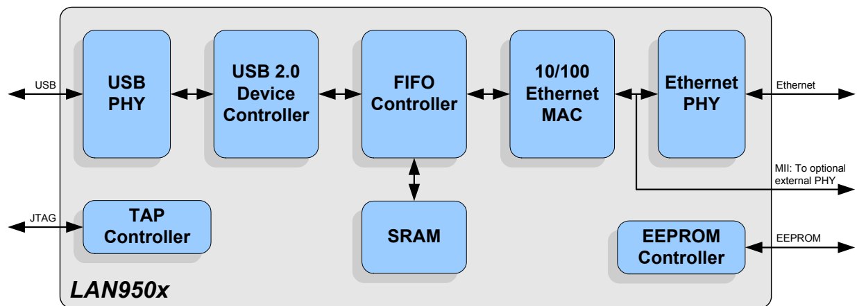
Figure 1 System Diagram
