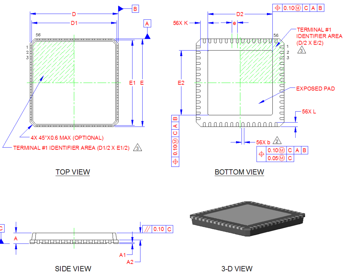
Figure 2 LAN950x 56-QFN Package
