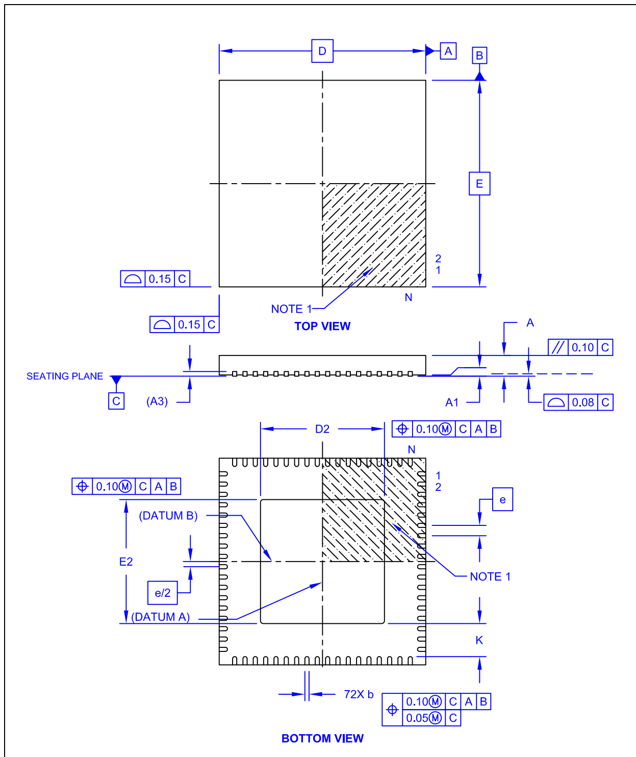
FIGURE 21-1: 72-QFN PACKAGE
