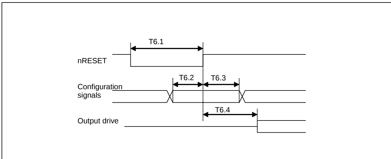
FIGURE 6-7: RESET TIMING
