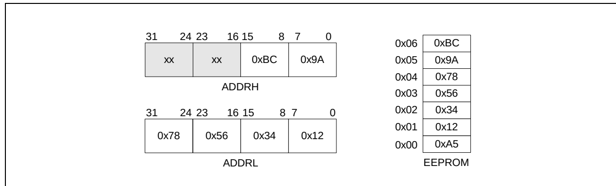
FIGURE 5-2: Example ADDR L , ADDR H and EEPROM Setup
