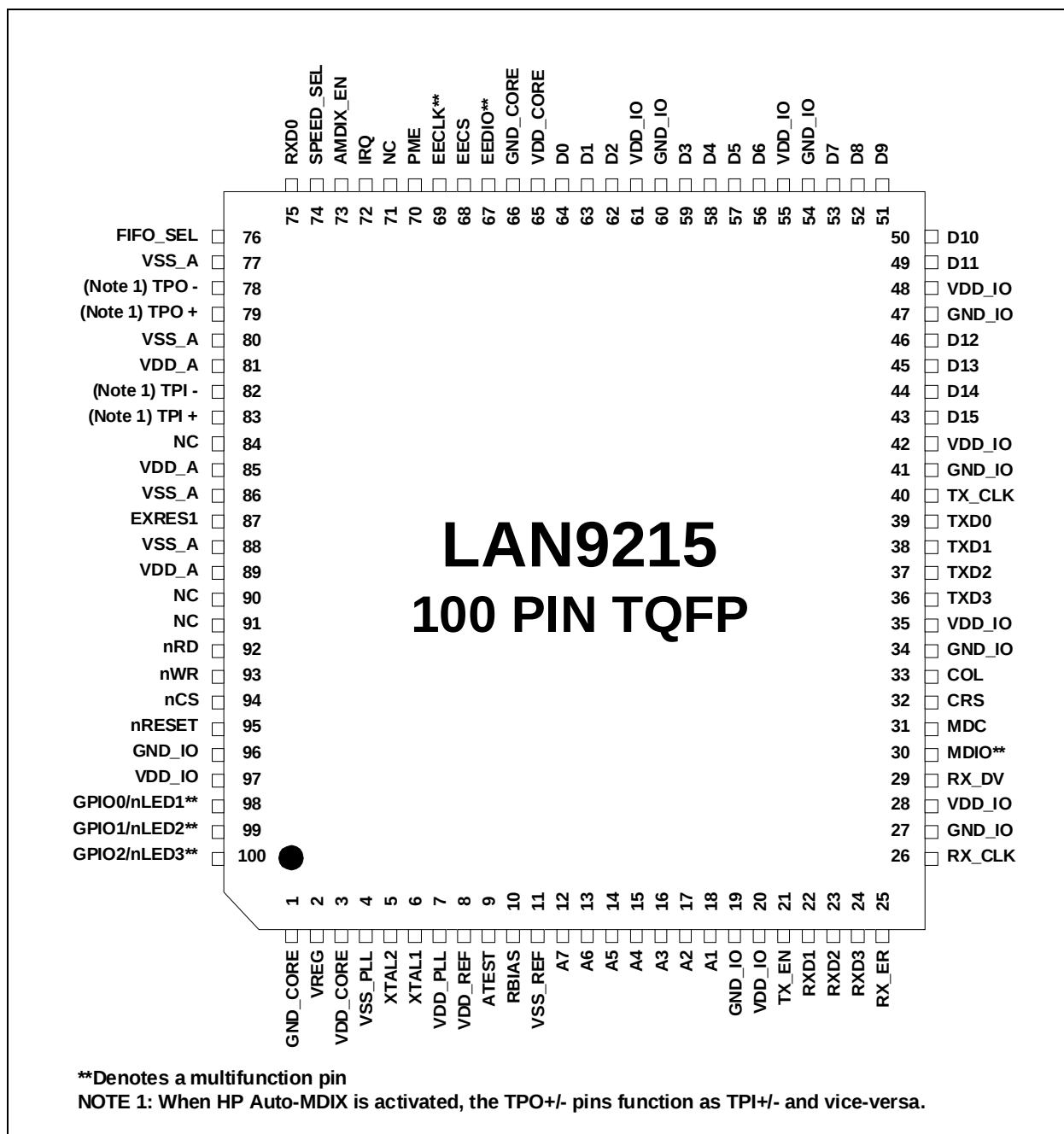
FIGURE 2-1: 100-TQFP PIN CONFIGURATION (TOP VIEW)
