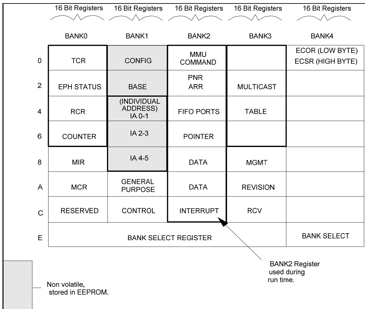
Figure 7.1 - LAN91C96i Registers
