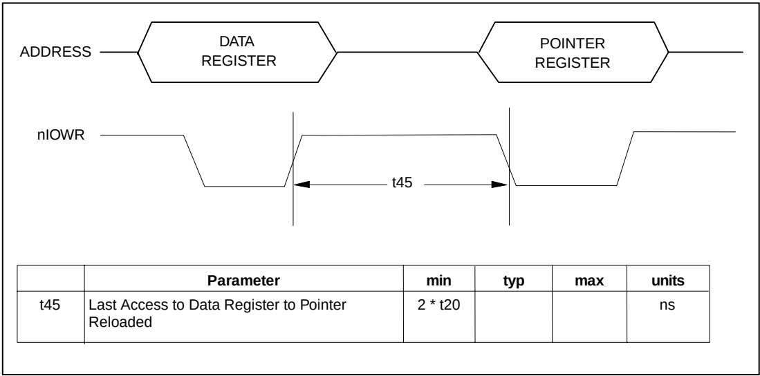
Figure 12.21 – Memory Write Timing
