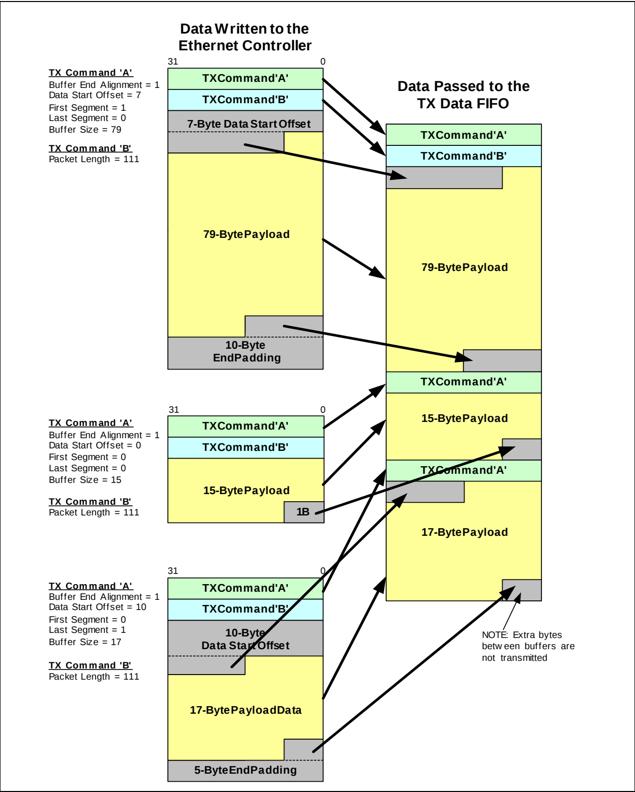
FIGURE 3-15: TX EXAMPLE 1
