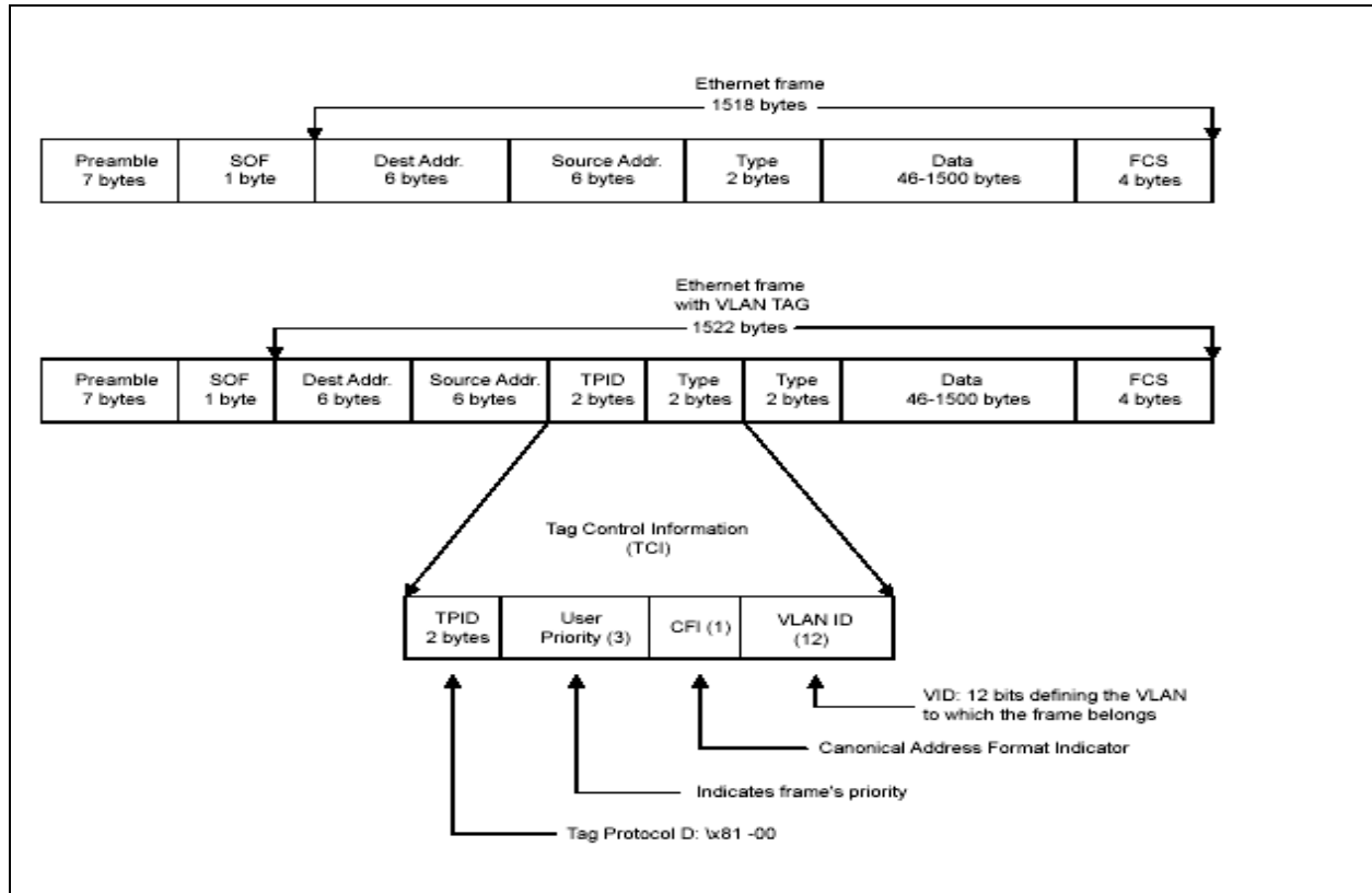
FIGURE 3-2: VLAN FRAME
