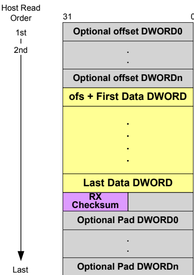
Figure 3.28 RX Packet Format with RX Checksum
