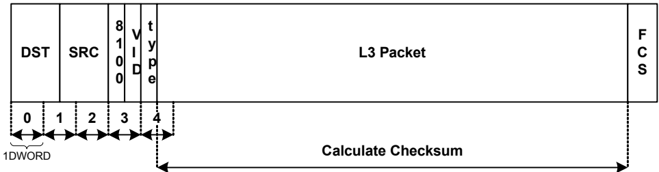
Figure 3.4 Ethernet Frame with VLAN Tag
