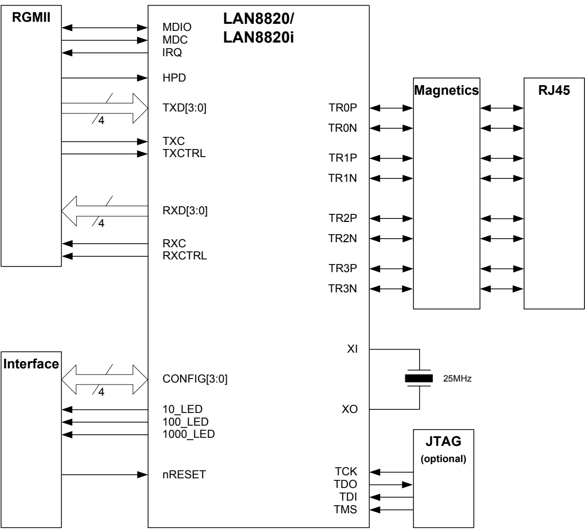
FIGURE 3-6: SIMPLIFIED APPLICATION DIAGRAM
