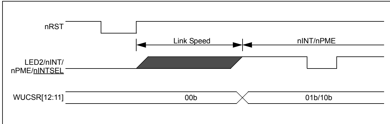
FIGURE 3-13: LED2/nINT/nPME WITH nINTSEL DISABLED
