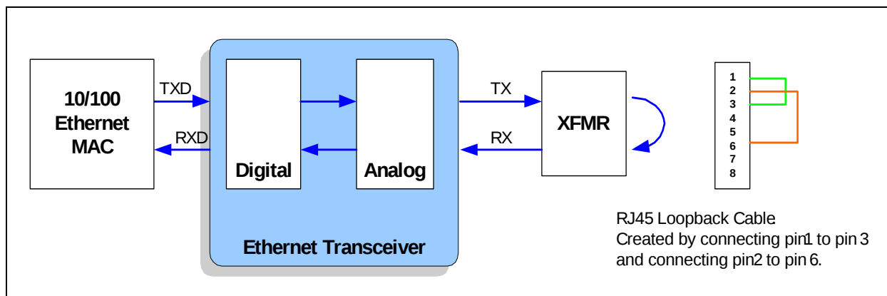
FIGURE 5-4: CONNECTOR LOOPBACK BLOCK DIAGRAM
