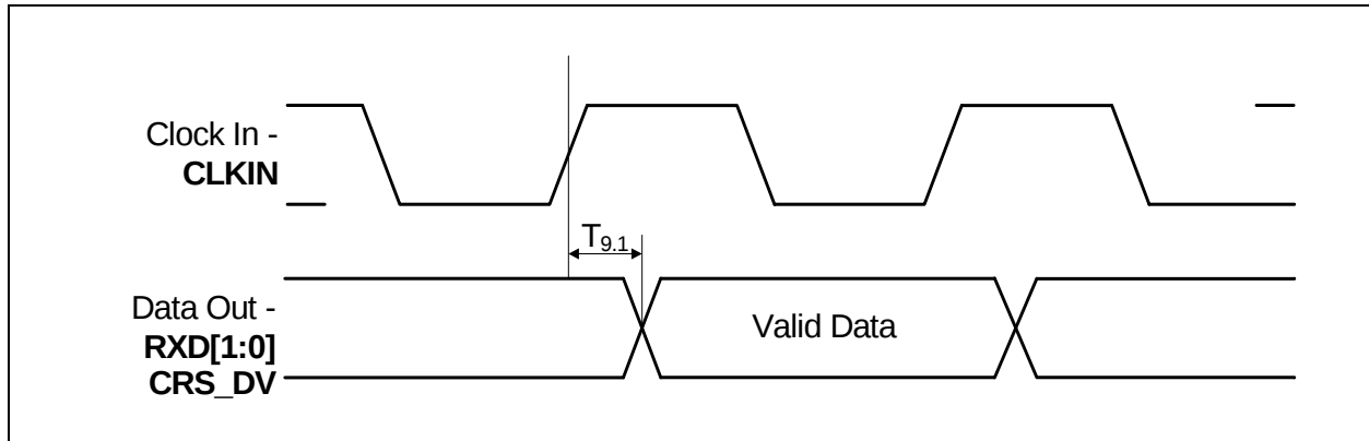
FIGURE 6-8: 10M RMII RECEIVE TIMING DIAGRAM
