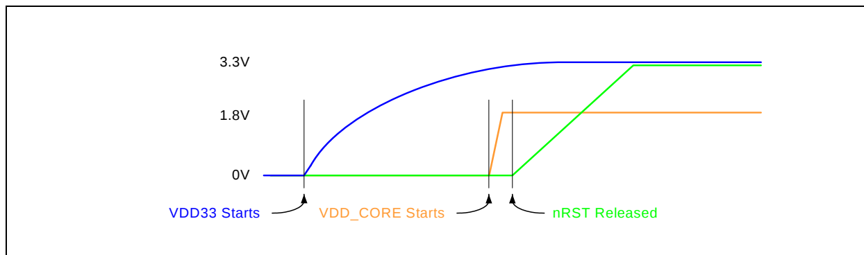
FIGURE 5-1: RESET TIMING DIAGRAM
