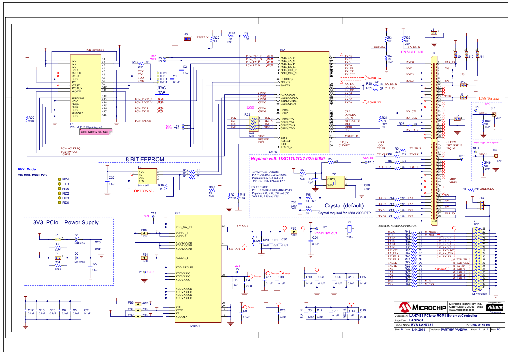
FIGURE B-1: LAN7431-EDS EVALUATION BOARD SCHEMATICS
