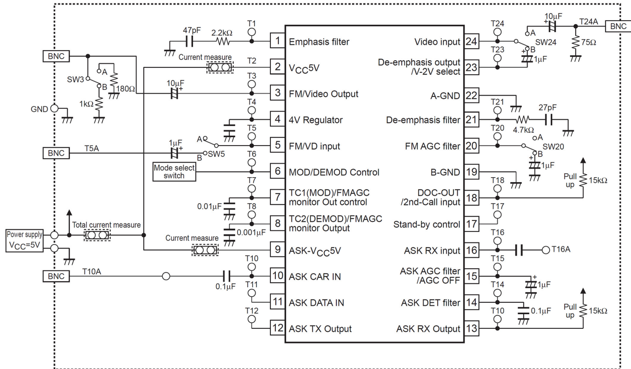
Figure 4. Test Circuit
