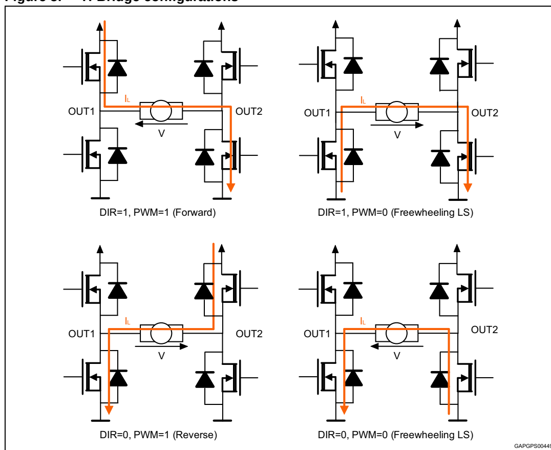
Figure 5. H-Bridge configurations
