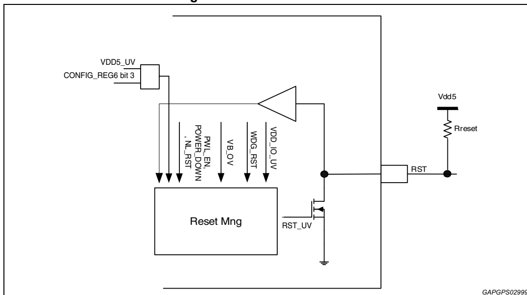
Figure 13. Smart reset circuit
