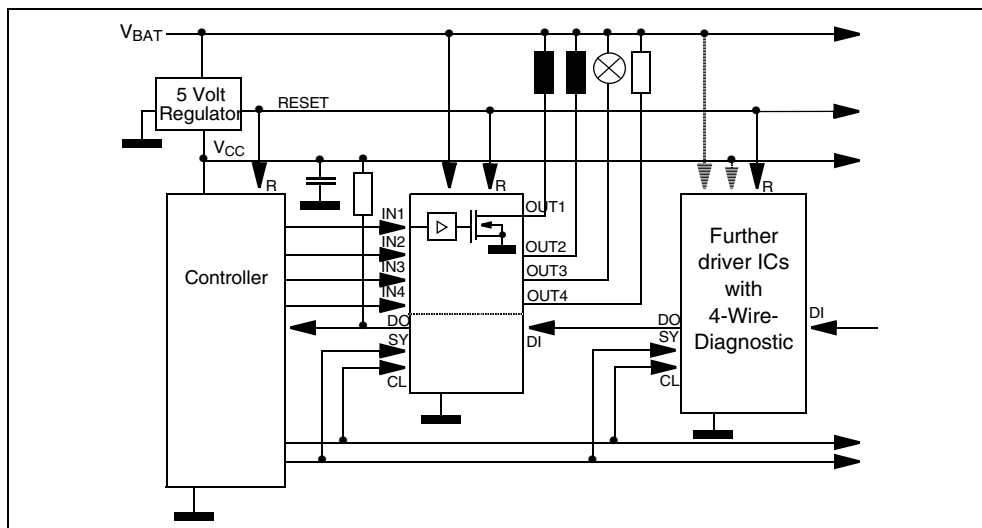
Figure 4. Application Circuit
