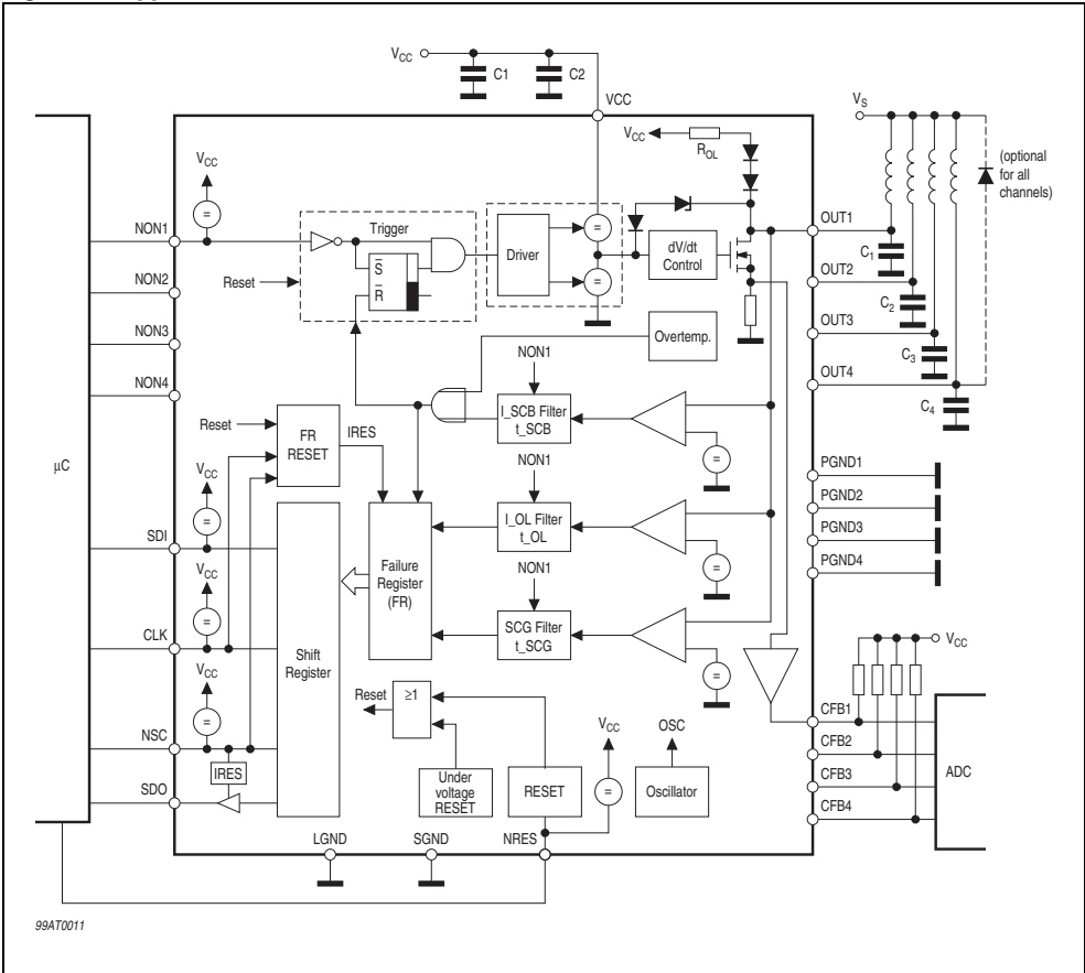
Figure 11. Application Circuit
