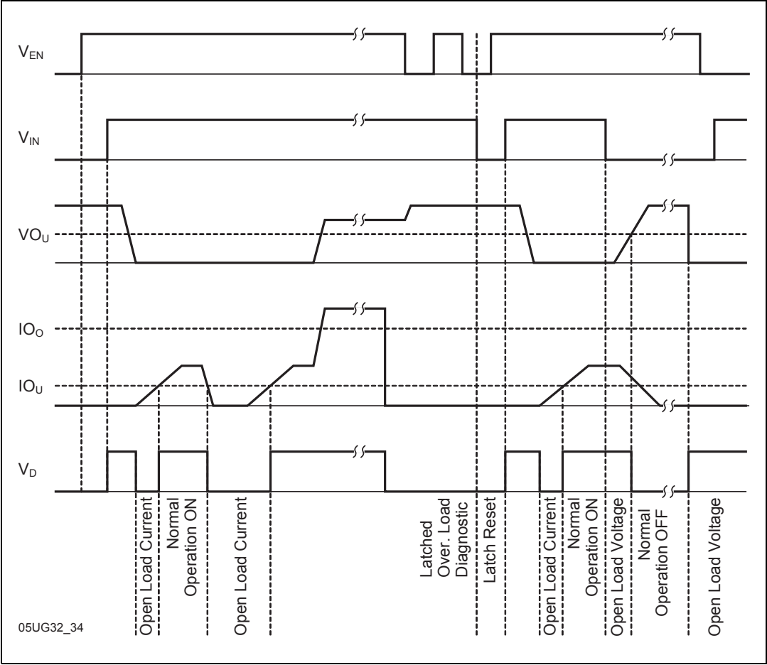
Figure 7. Logic diagram
