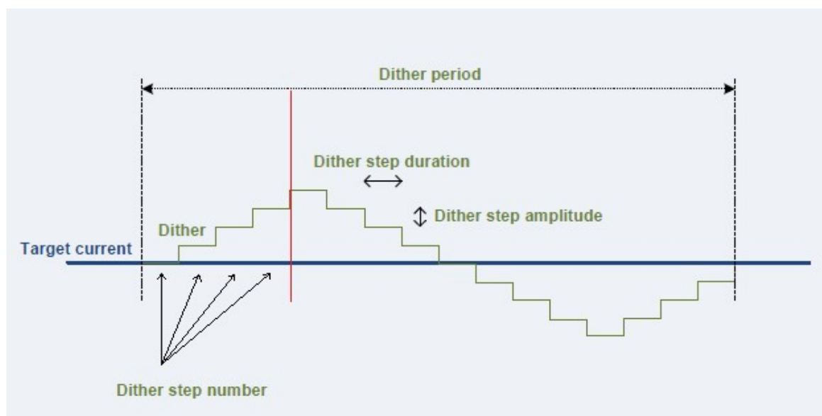
Figure 29. Dither functionality
