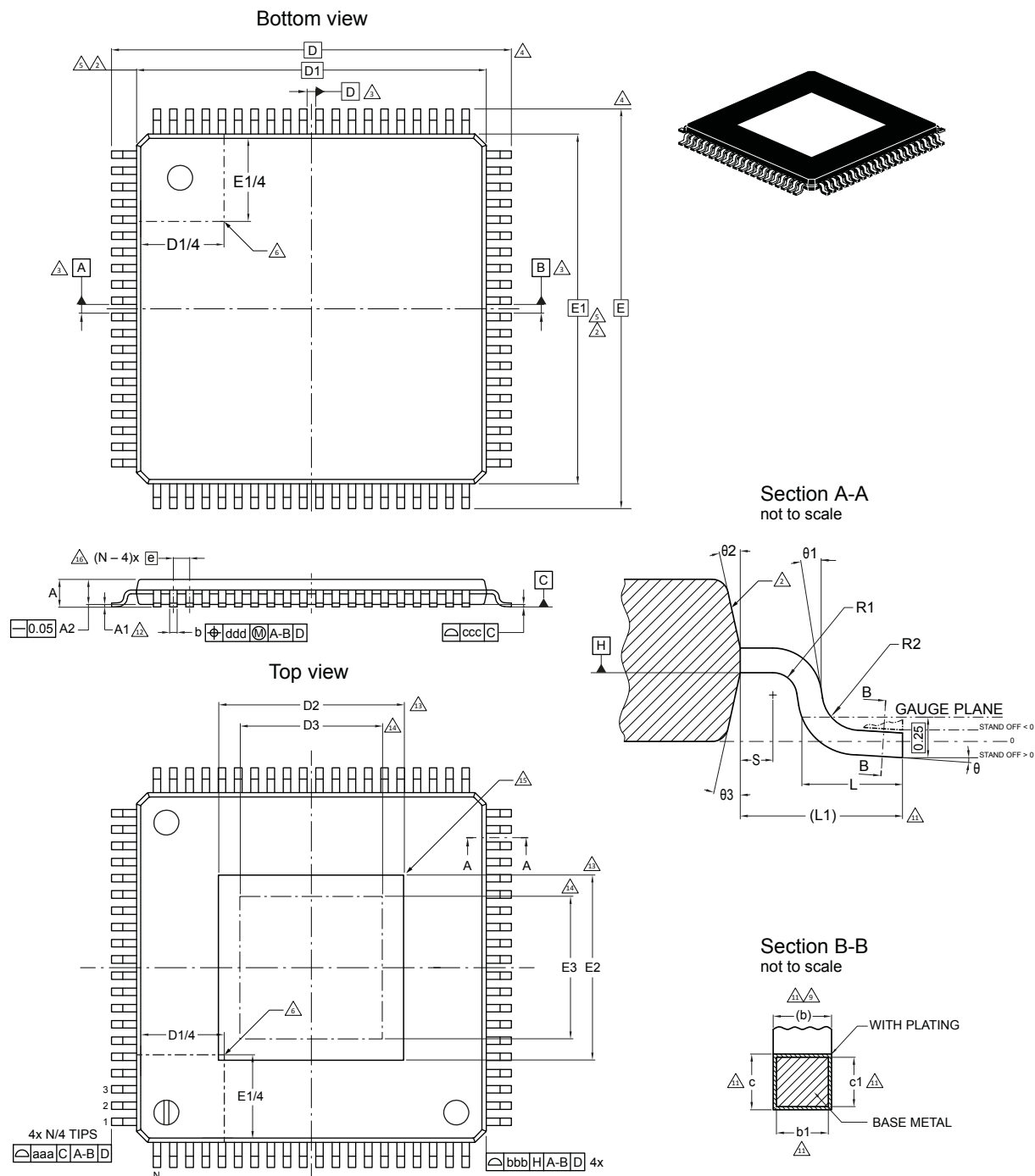
Figure 72. TQFP80 (14x14x1 mm. exp. pad up) package outline
