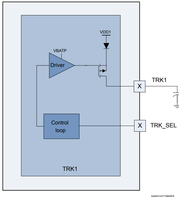
Figure 14. TRK regulators
