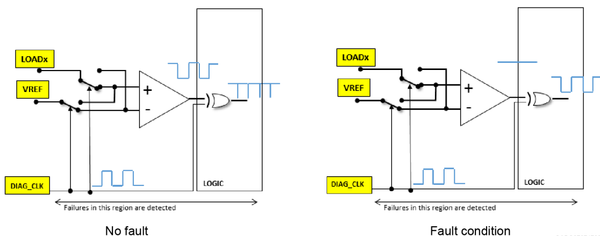
Figure 69. Diagnostic analog self test basic implementation
