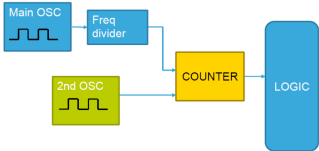
Figure 65. Oscillator monitor
