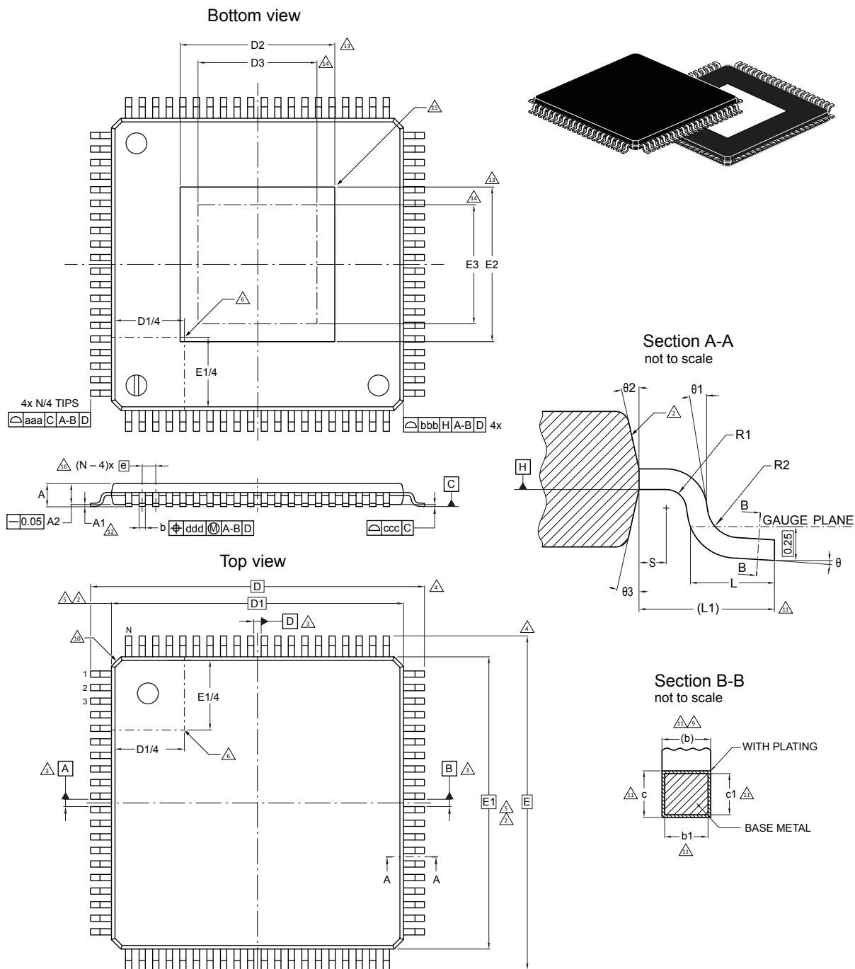
Figure 74. TQFP80 (14x14x1 mm. exp. pad down) package outline
