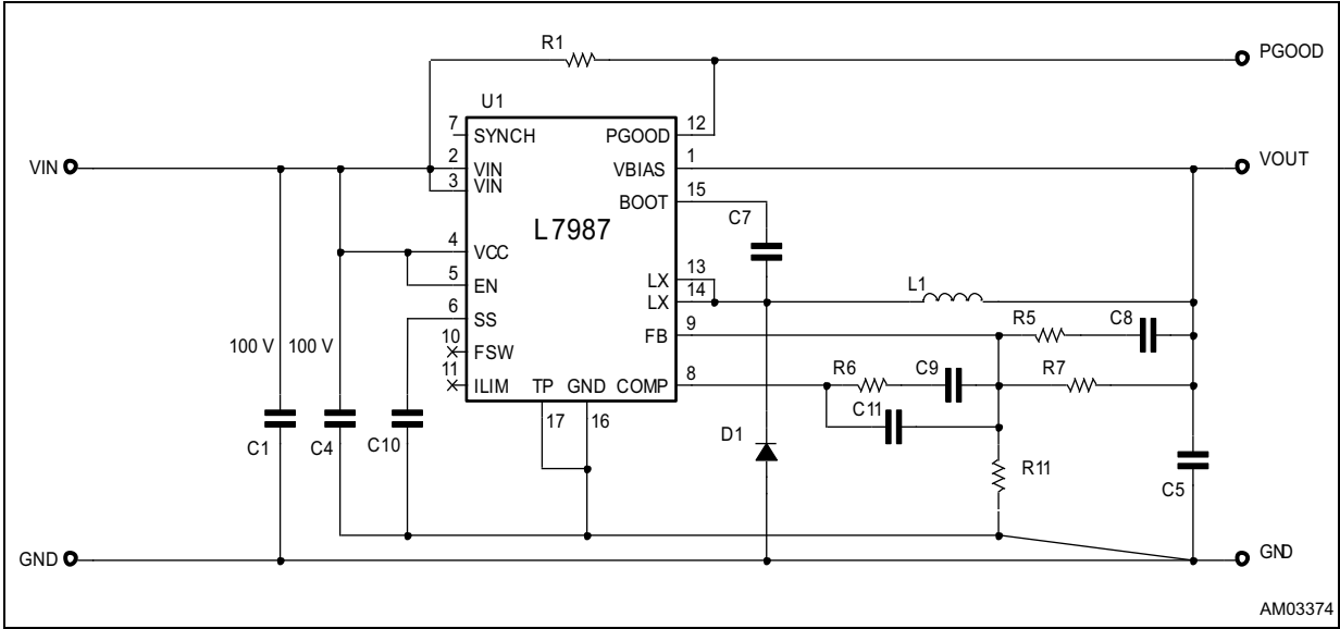
Figure 1. Application schematic
