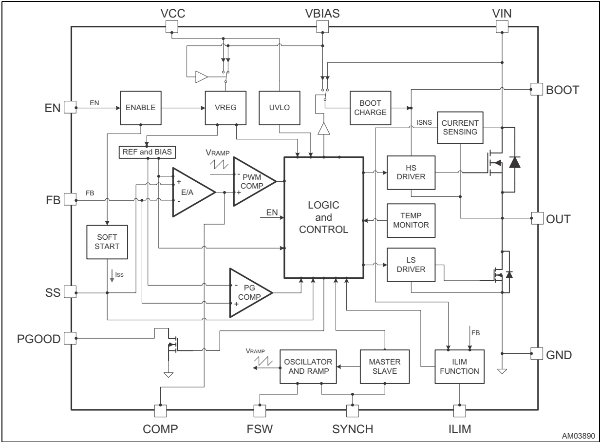
Figure 2. Block diagram
