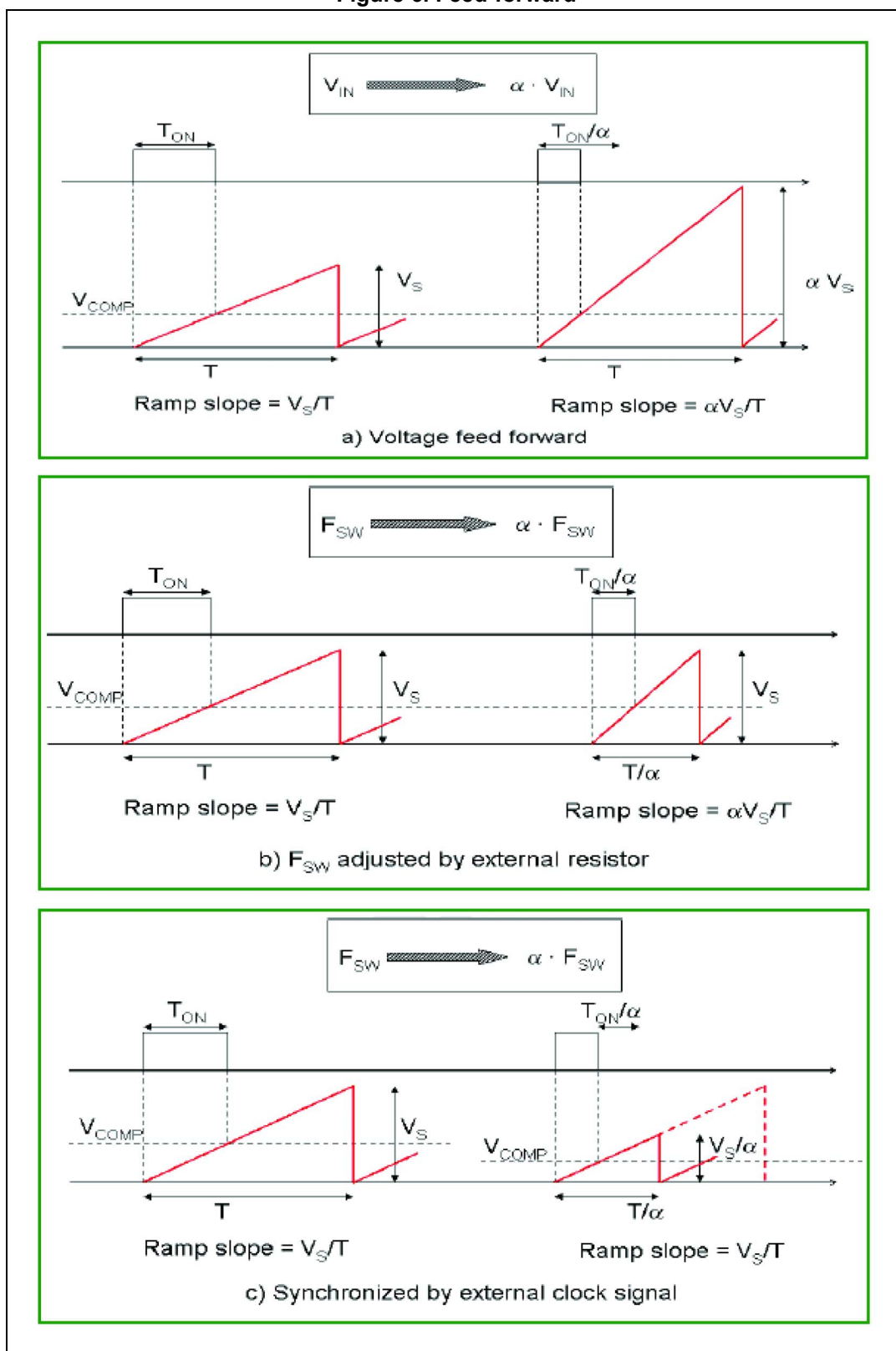
Figure 6. Feed-forward
