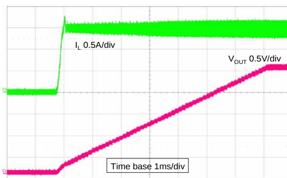
Figure 31. Soft-start
