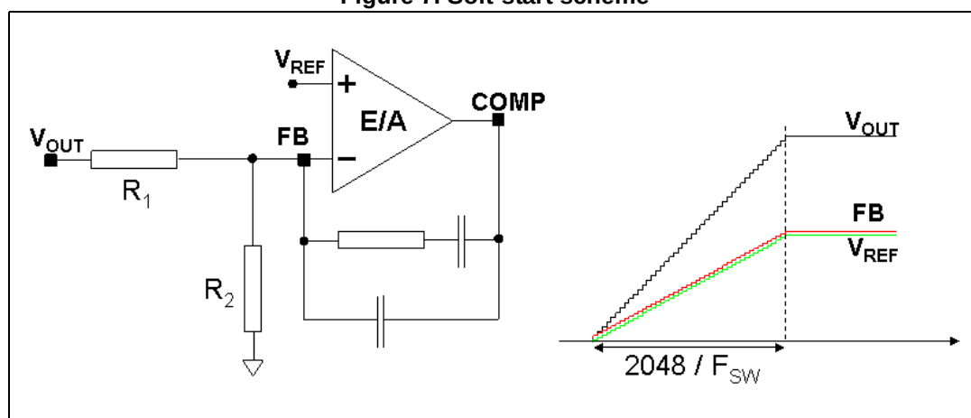
Figure 7. Soft-start scheme
