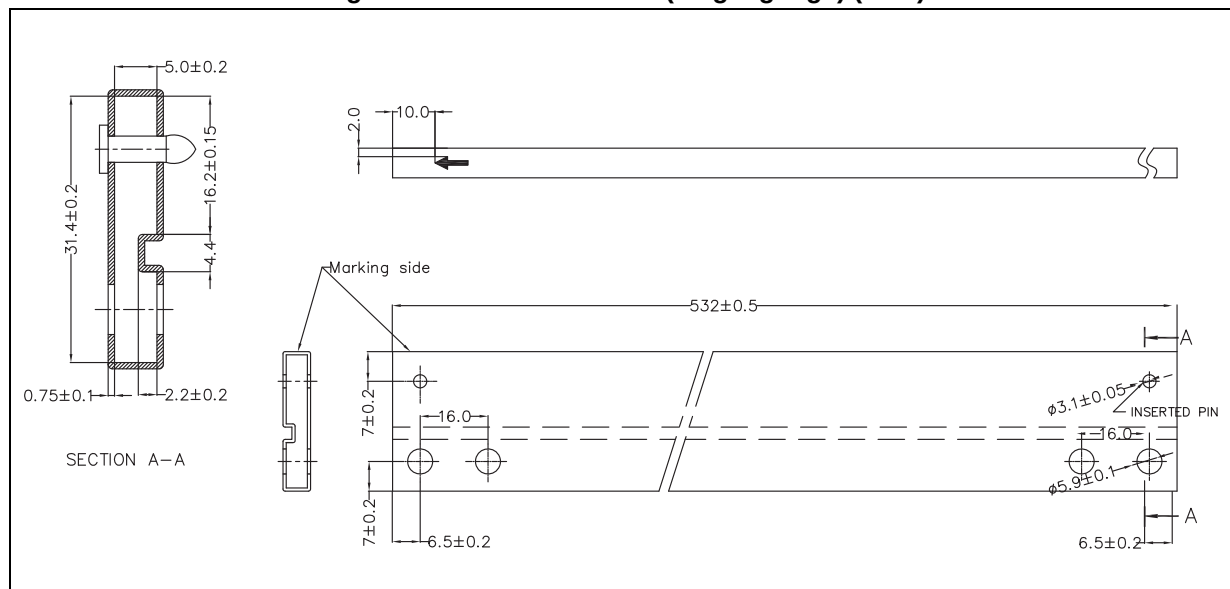
Figure 46. Tube for TO-220 (single gauge) (mm.)
