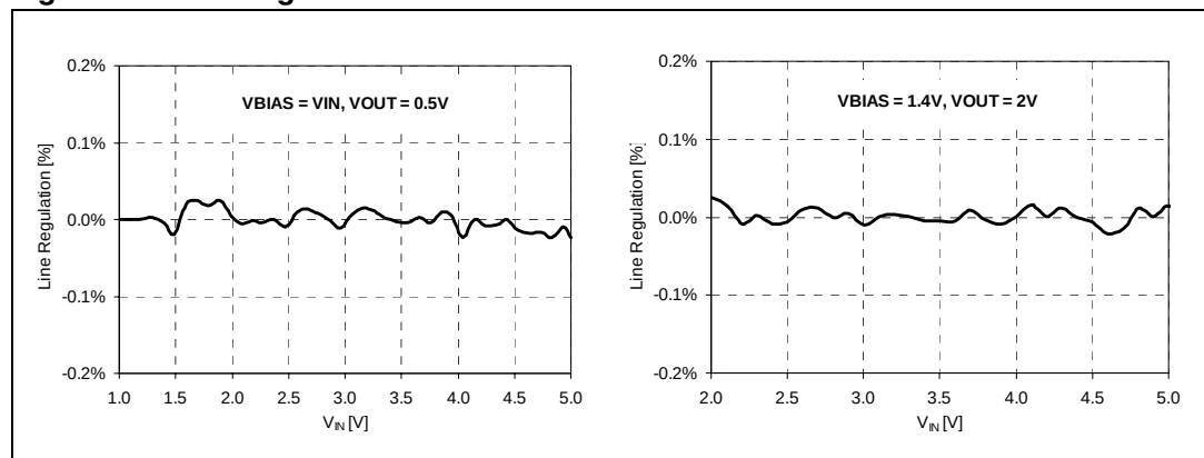
Figure 7. Line regulation
