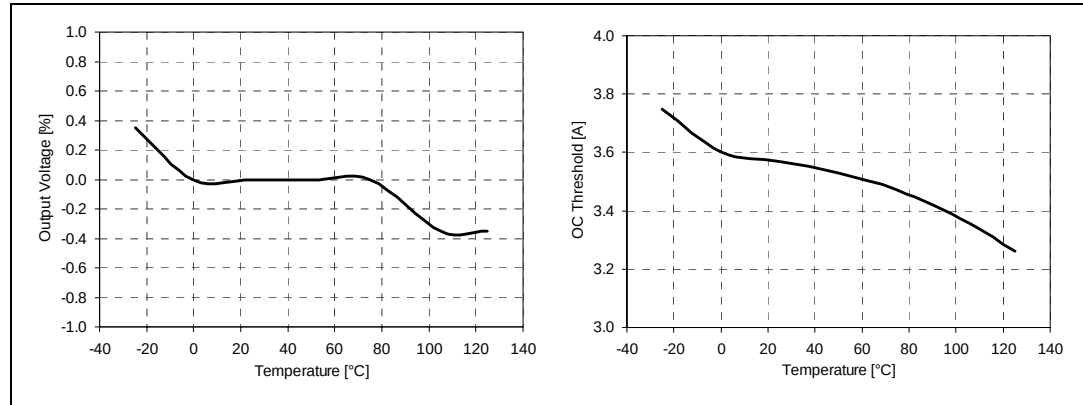
Figure 6. Quiescent and shutdown current vs junction temperature
