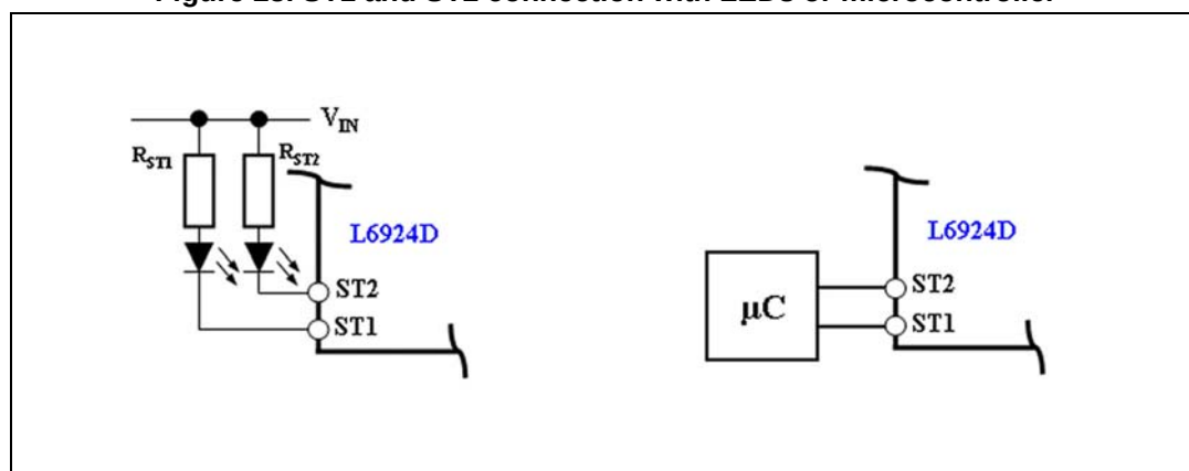
Figure 23. ST1 and ST2 connection with LEDs or microcontroller
