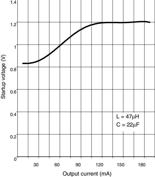
Figure 5. Startup Voltage vs Output Current
