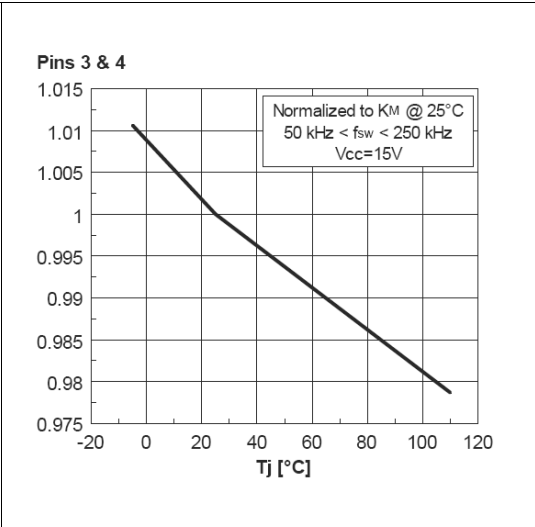
Figure 14. OCP delay thresholds vs junction temperature
