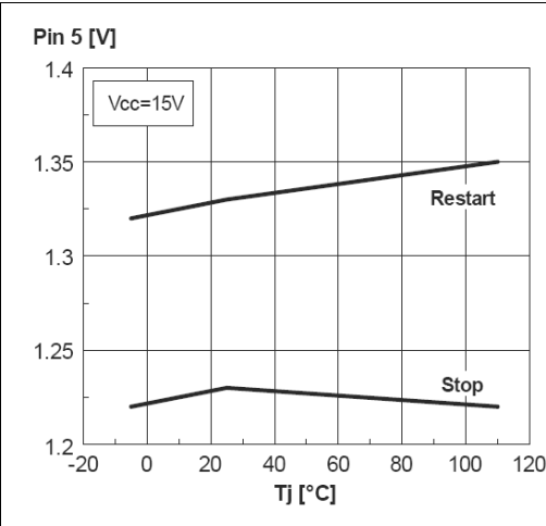
Figure 17. Line thresholds vs junction temperature
