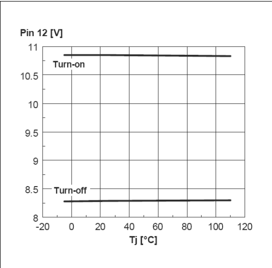
Figure 6. UVLO thresholds vs junction temperature
