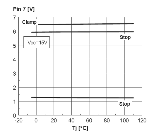
Figure 19. Latched disable threshold vs junction temperature
