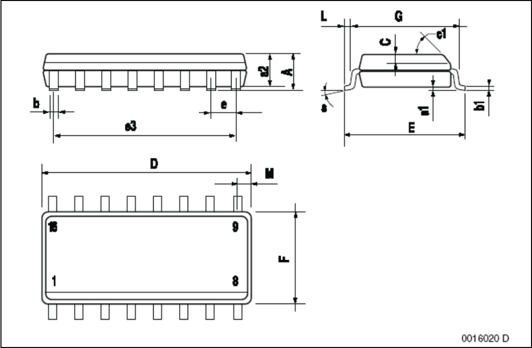
Figure 36. Package dimensions
