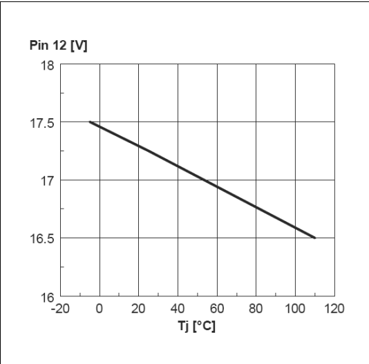
Figure 5. VCC clamp voltage vs junction temperature
