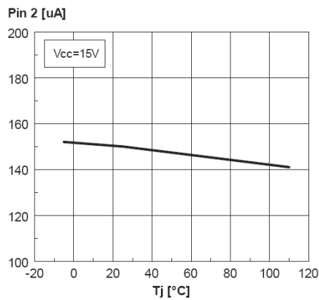
Figure 13. OCP delay source current vs. junction temperature
