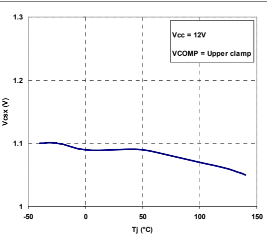
Figure 12. V_{cs} clamp vs T_J
