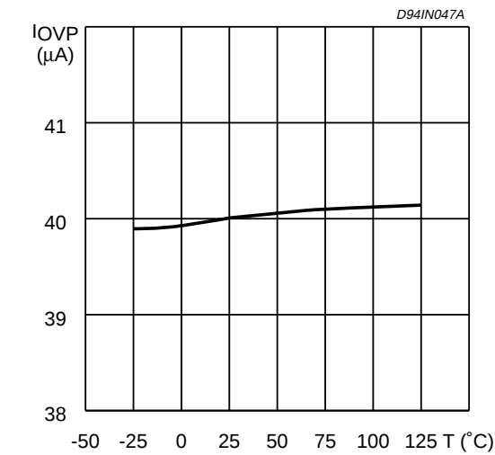
Figure 11. OVP Current Threshold vs. Temperature
