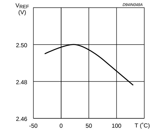
Figure 14. Voltage Feedback Input Threshold vs. Temperature
