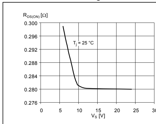
Figure 33. Typical low-side R_{DS(ON)} vs. supply voltage
