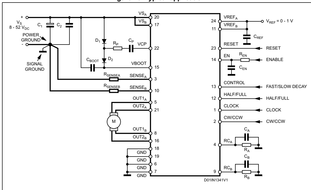
Figure 25. Typical application
