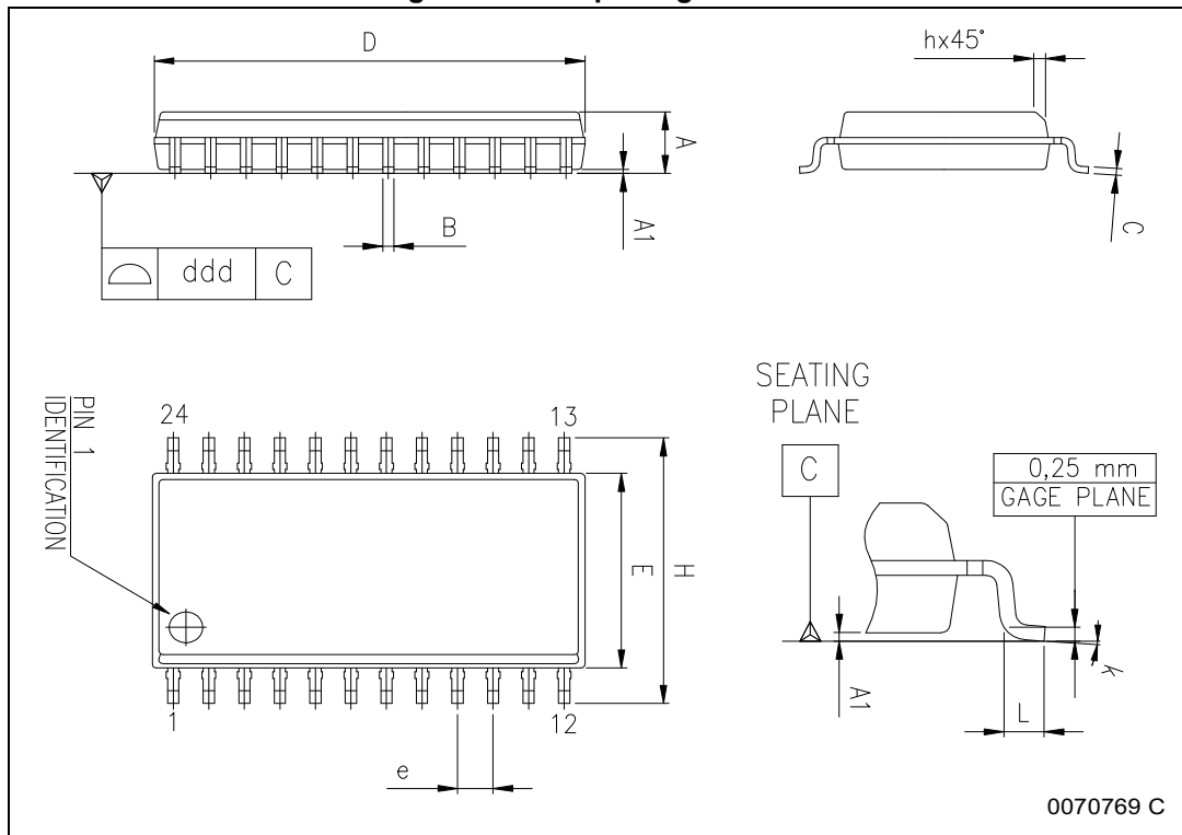
Figure 6. SO24 package outline
