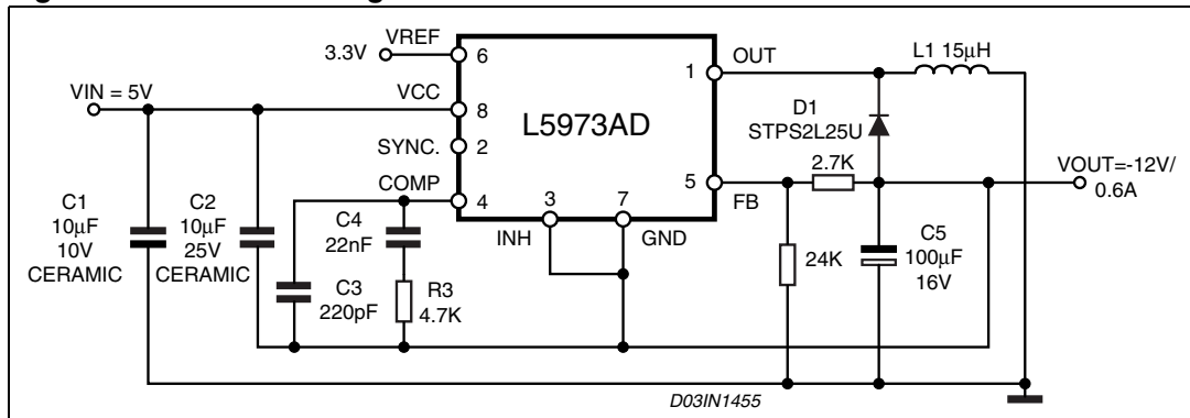
Figure 13. Buck-Boost regulator
