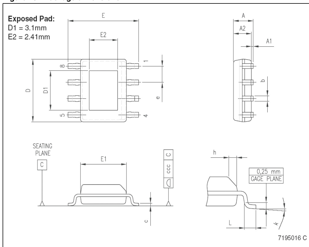
Figure 15. Package dimensions
