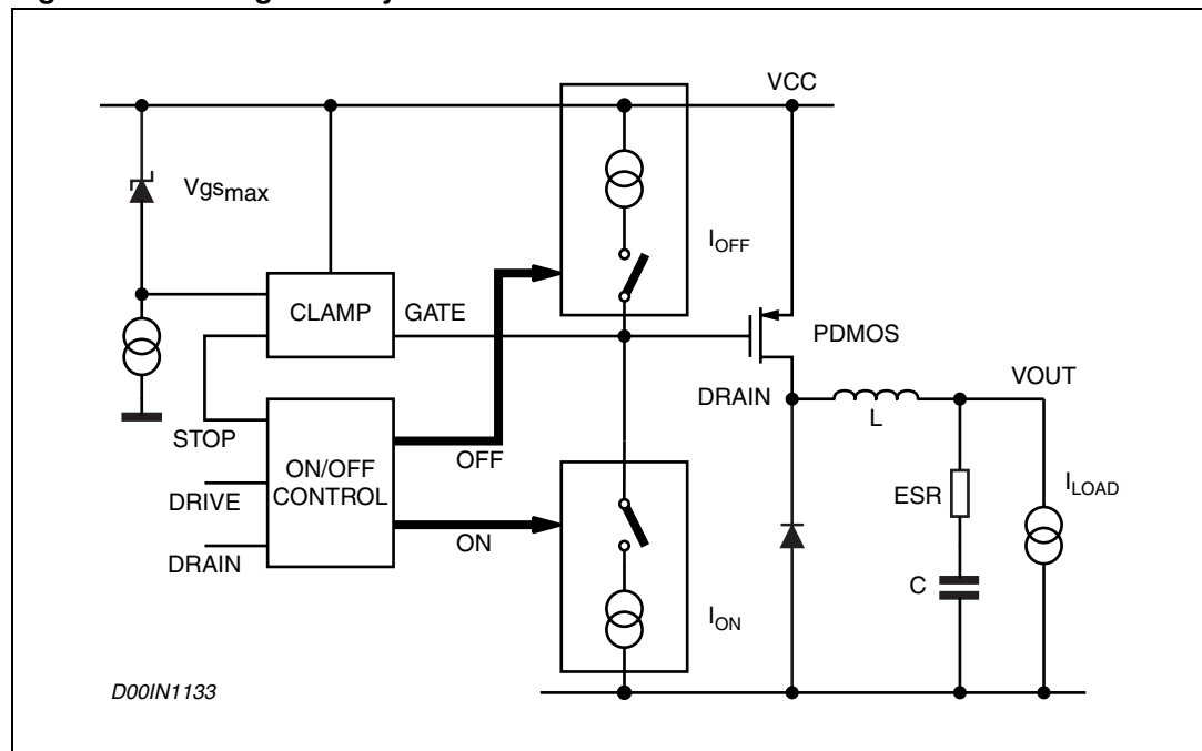
Figure 6. Driving circuitry
