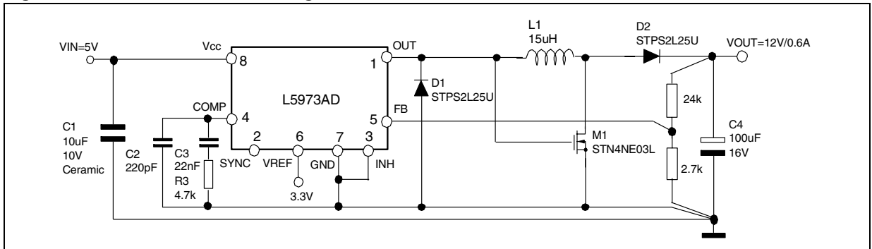
Figure 15. Buck-Boost regulator
