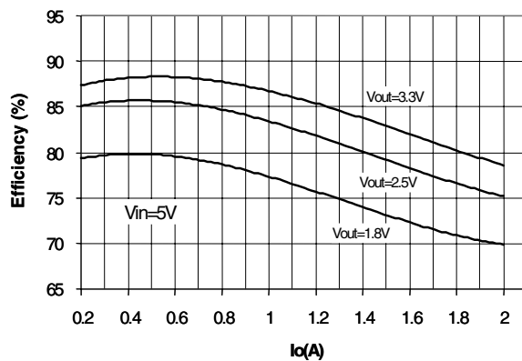
Figure 13. Efficiency vs. Output Current
