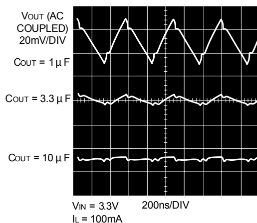
Output Ripple
