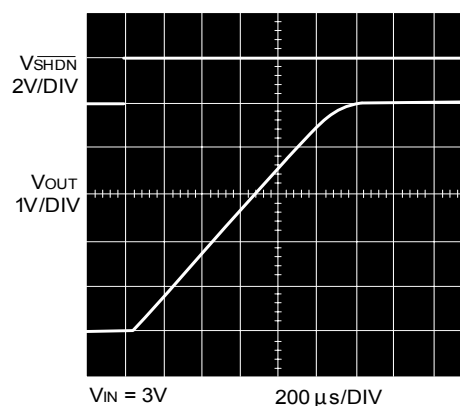
V OUT Soft-Start Ramp
