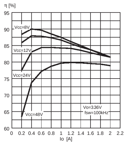
Figure 14. Efficiency vs. output current.
