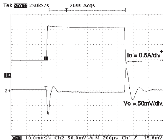
Figure 21. Load transient.
