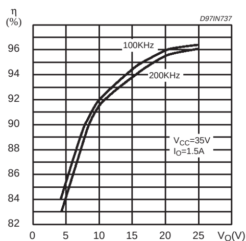
Figure 12. Efficiency vs output voltage.
