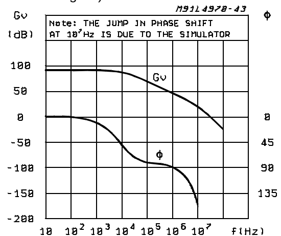
Figure 31: Open Loop Frequency and Phase Response of Error Amplifier (see fig.7C)
